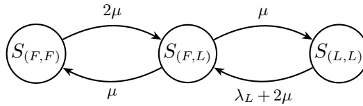
Figure 3 Three-state CTMCs for the joint freshness of two units of the same product sharing the shelf under the conventional model.
