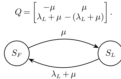
Figure 1 Two-state CTMC for the freshness of the product at store.
