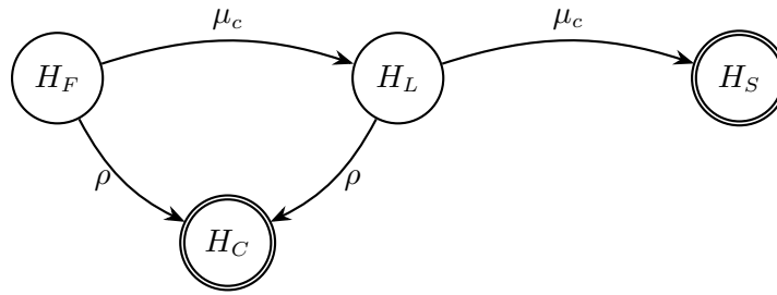
Figure 2 Four-state CTMC for a purchased unit at a household.
