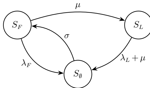
Figure 5 Three-state CTMC for a single product under non-immediate restocking.
