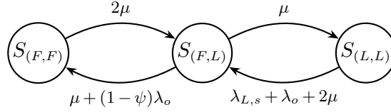
Figure 4 Three-state CTMC for the joint freshness of two units of the same product sharing the shelf under the omnichannel model.
